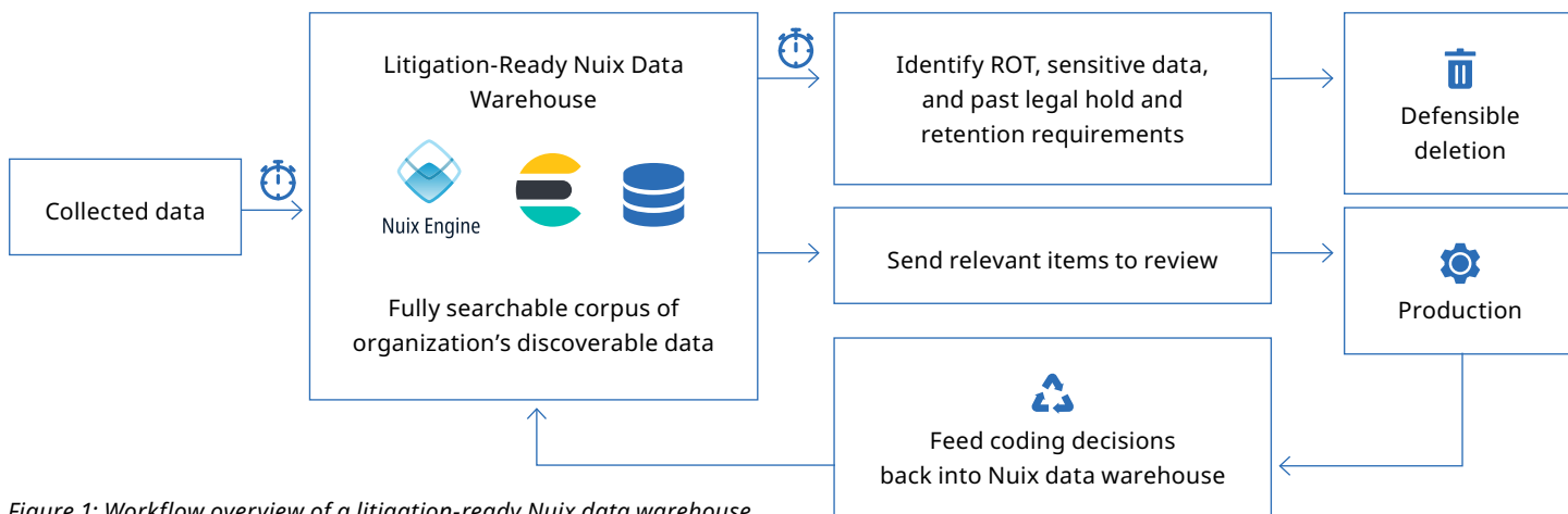
Figure 1: Workflow overview of a litigation-ready NUIX data warehouse.
